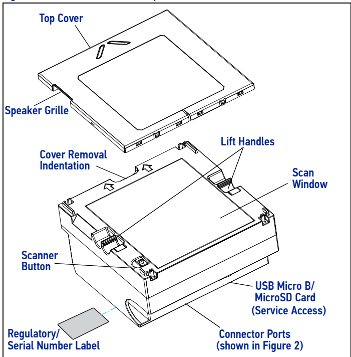
Figure 1. Scanner Features - Top View
